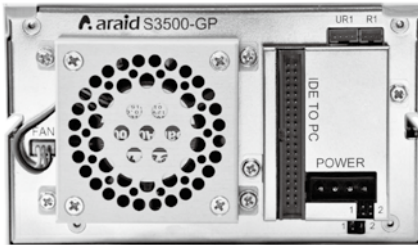
Rear View of ARAID 3500-HIDE / S3500-HIDE
